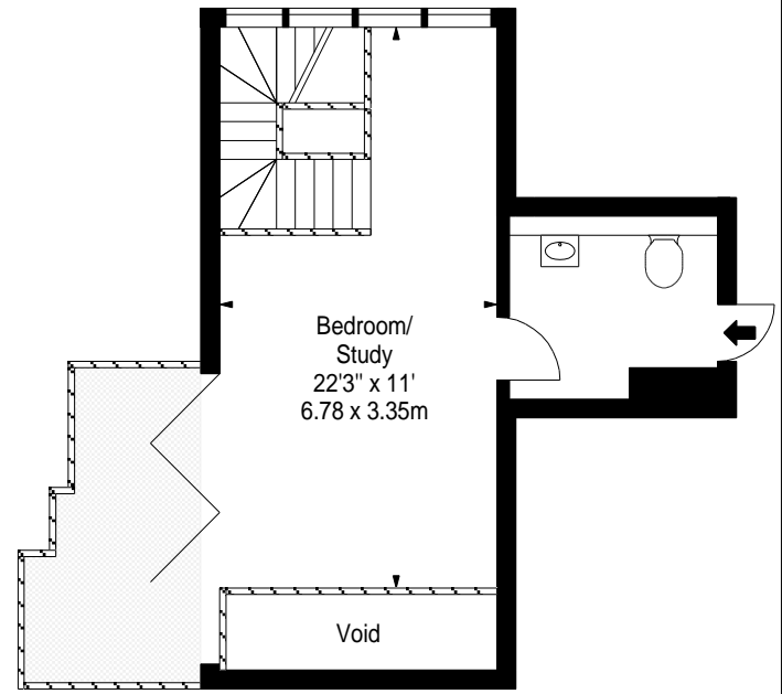
FIFTH FLOOR
